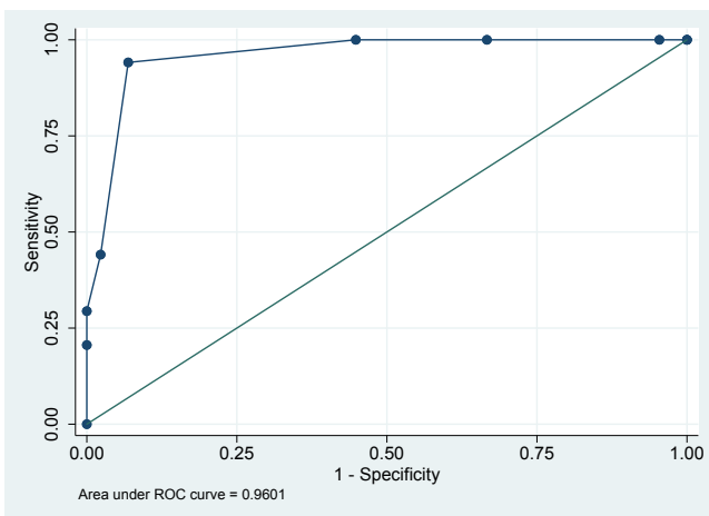
Fig. 1. ROC Curve
